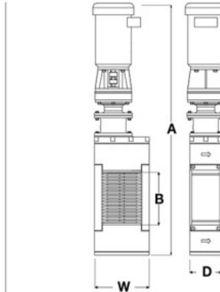
SHRED-H - Hopper Configuration
